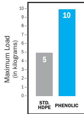
ASTM D 2197-98(2002) Scratch Resistance
