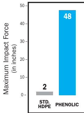
ASTM D 2794-93(1999)e1 Impact Resistance
