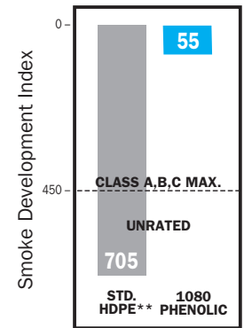
ASTM E 84-01* Surface Burning Characteristics (lower values are superior)
