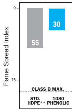
ASTM E 84-01* Surface Burning Characteristics (lower values are superior)
