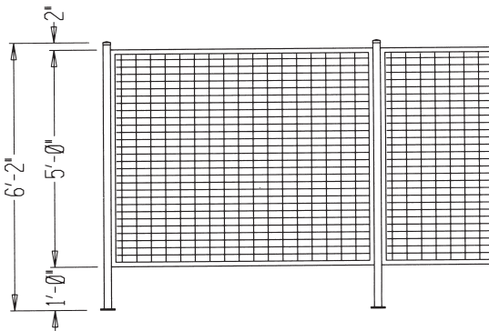
TYPICAL ELEVATION
