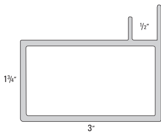
HSW-SBC Series Frames
