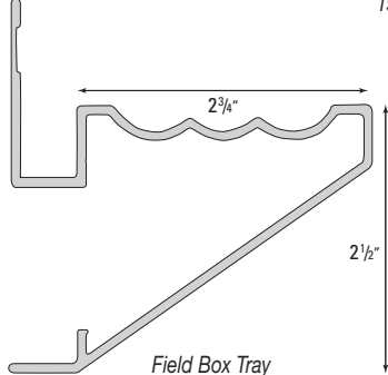
Field Box Tray
