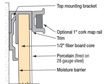
Walker Headliner detail (see page 22 for additional maprail and accessories).
