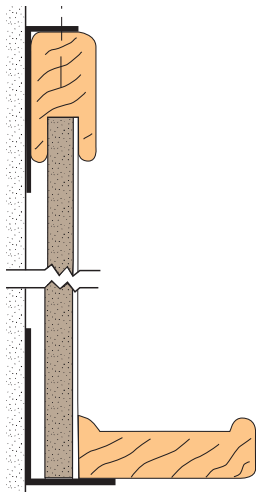
Detail wood markerboard with tray
