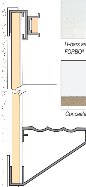
Marker or chalkboard detail with 1" maprail and box tray with cast endcaps
