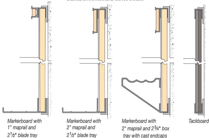
Standard Architectural Series Details
