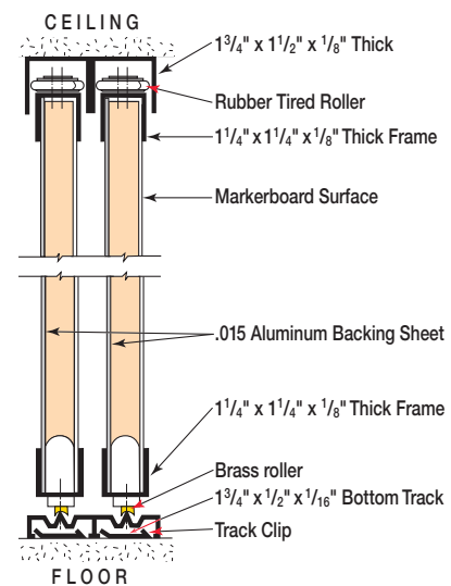
2-Track Unit illustrated (tracks sold separately)
