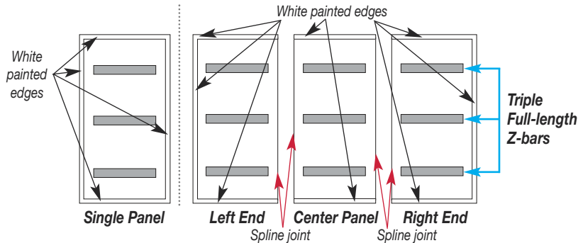
Square Corner Painted Edge
